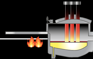
Consteel EAF
